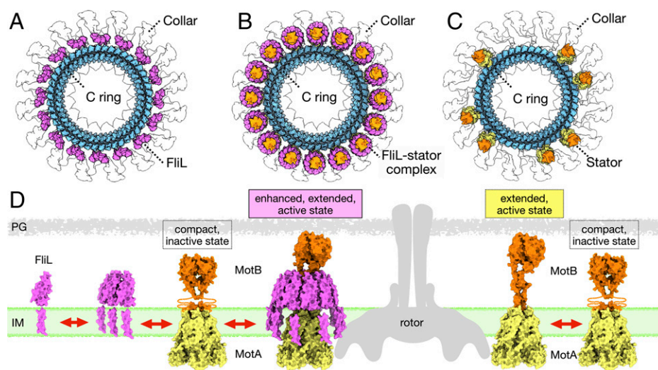
Fig. 5. Maximal torque generation by the flagellar motor requires proper assembly of the FliL–stator complex. (A) A top view of the \Delta motB motor. The FliL units that form partial rings are colored magenta, the collars are transparent, and the C ring subunits are colored cyan. (B) A top view of the WT motor. The 16 BbFliL rings surrounding the stators (MotB subunits colored orange) are colored magenta, the collars are transparent, and the C ring subunits are colored cyan. (C) A top view of the \Delta fliL motor. In the absence of the BbFliL rings, the motor is surrounded by fewer stator complexes. (D) A model for the assembly of the FliL–stator supramolecular complex necessary for maximizing torque generation by the bacterial flagellar motor. Left of the schematics for the rotor, FliL units interact with themselves to form oligomers that will interact with the active stator units. Interactions between FliL oligomers and the stator units result in the cooperative assembly of the FliL–stator supramolecular complex around the rotor. Right of the schematics for the rotor, comparison between the stator in its active, extended conformation in the absence of FliL (Left) and stator in its inactive form. Double-headed arrows with a dotted line indicate MotB PGB binding to and dissociation from the peptidoglycan layer.
