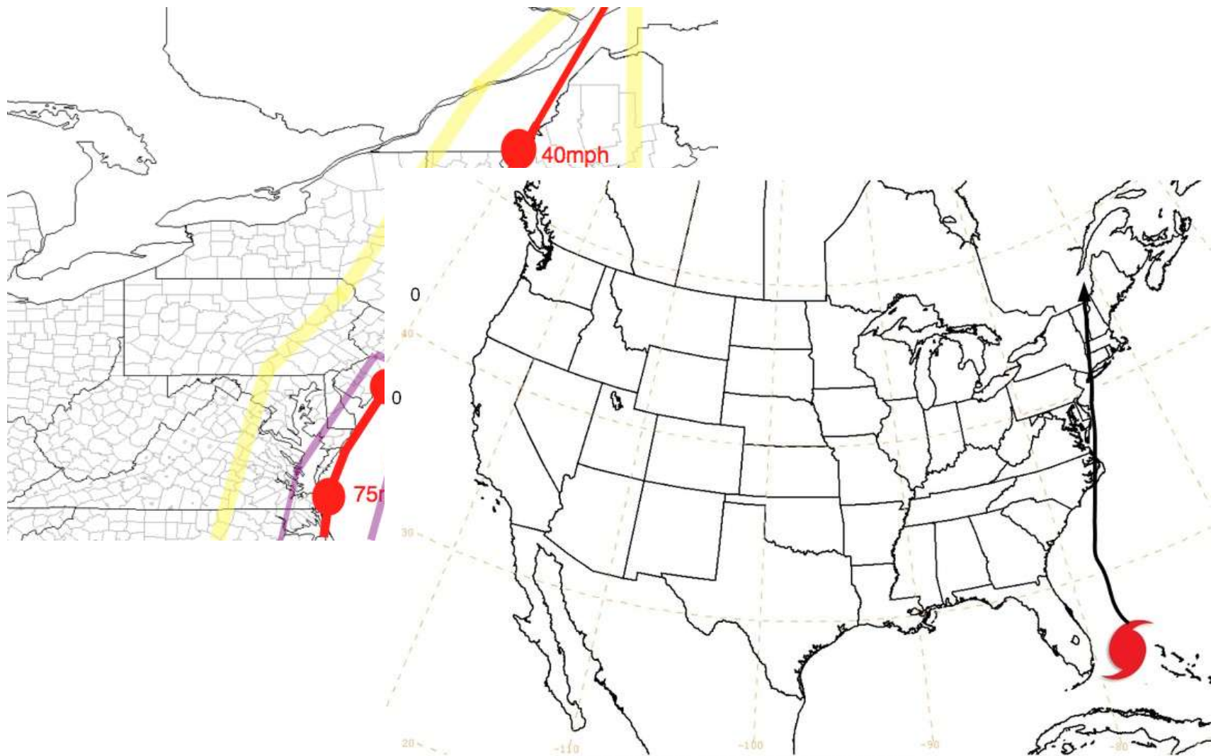
Hurricane Irene track forecast
