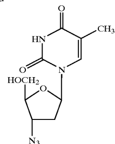
2',3'-dideoxy-3'-azidothymidine (also 3'-azido-3'-deoxythymidine) (AZT)
