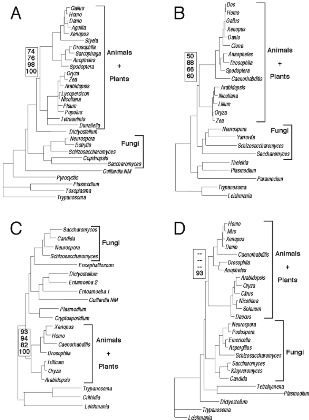
Fig. 2 Phylogenetic trees recovered from Bayesian inference of four examples of genes that provide support for an animal/plant grouping (A) PCNA , (B) CKII \alpha , (C) CEG , (D) CIT . Support values are, in descending order, from parsimony bootstrap, neighbor-joining bootstrap, quartet-puzzling maximum-likelihood and Bayesian inference. Values below 50% are indicated by (—). In addition to sequences from the nine complete genomes used in Fig. 1, the following sequences were retrieved by reciprocal tBLASTn searches for each data set. (A) Gallus gallus AB053163, Danio rerio BC049535, Aguilla japonica AB025357, Xenopus laevis BC041549, Styela clava L42763, Sarcophaga crassipalpis AF020427, Anopheles gambiae XM319407, Spodoptera frugiperda AB069854, Zea mays AY110234, Lycopersicon esculentum AJ515474, Nicotiana tobacum AB025029, Pisum sativum Y16796, Populus nigra AB041506, Tetraselmis chui AF012212, Dunaliella tertiolecta AF034201, Neurospora crassa XM331630, Botrytis cinerea AL117064, Coprinopsis cinereus AB056666, Guillardia theta NM AF083031, Pyrocystis lunula AF508260, Toxoplasma gondii AF242301; (B) Bos Taurus M93665, G. gallus M59456, X. laevis X62375, D. rerio BC044403, Ciona intestinalis AY092081, A. gam-
