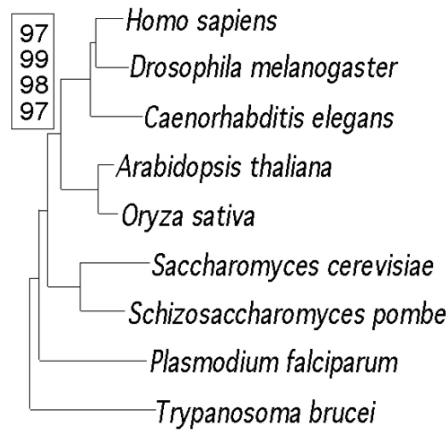
Fig. 1 Identical tree recovered from parsimony bootstrap (33), neighbor-joining bootstrap (33), quartet-puzzling maximum-likelihood (34) and Bayesian inference (35), with respective support values for the animal/plant grouping, on a combined alignment of 2,757 inferred amino acids from nine genes. These genes were chosen based on previously published analyses indicating that they contain a tree-building signal favoring animals + plants (5, 6, 11); to permit the most reliable estimate of orthologous relationships, only completed genomes were sampled for this analysis. The nine sequences are capping enzyme guanylyltransferase ( CEG ), casein kinase II alpha subunit ( CK-II \alpha ), citrate synthase ( CIT ), enolase, F-ATPase \beta , 70 kD heat shock protein ( HSP70 ), 90 kD heat shock protein ( HSP90 ), proliferating-cell nuclear antigen ( PCNA ) and triosphosphate isomerase ( TPI ).
