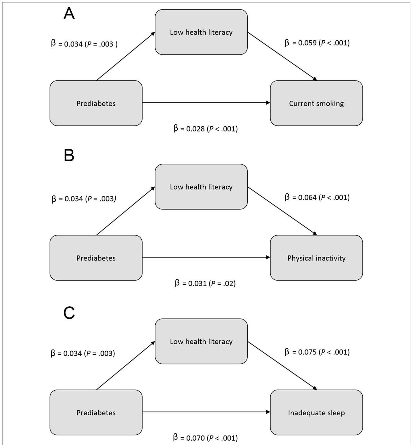
Figure 2. Results of path analysis in a study (N = 54 344 adults aged \geq 18 ) on health literacy and health behaviors among adults with prediabetes, 2016 Behavioral Risk Factor Surveillance System survey. 13 (A) Relationship among prediabetes, low health literacy, and current smoking. (B) Relationship among prediabetes, low health literacy, and physical inactivity. (C) Relationship among prediabetes, low health literacy, and inadequate sleep. Low health literacy was defined as answering “somewhat difficult” or “very difficult” to any of the 3 questions on obtaining information, understanding physicians, and understanding written information. Current smokers were defined as everyday smokers or some-day smokers; not current smokers were defined as former smokers or never smokers. Physical inactivity was coded according to the following yes/no question: “During the past month, other than your regular job, did you participate in any physical activities or exercises such as running, calisthenics, golf, gardening, or walking for exercise?” Inadequate sleep was coded according to the question, “On average, how many hours of sleep do you get in a 24-hour period?” Those who reported <7 hours were classified as having inadequate sleep. 17 Arrows indicate a direct effect.
