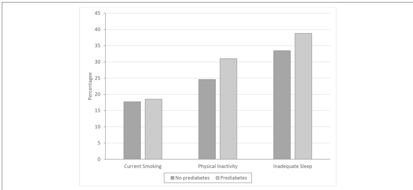
Figure 1. Health behaviors reported by respondents (54 344 adults aged \geq 18 ), by prediabetes status, 2016 Behavioral Risk Factor Surveillance System survey. 13 Current smokers were defined as everyday smokers or some-day smokers; not current smokers were defined as former smokers or never smokers. Physical inactivity was coded according to the following yes/no question: “During the past month, other than your regular job, did you participate in any physical activities or exercises such as running, calisthenics, golf, gardening, or walking for exercise?” Inadequate sleep was coded according to the question, “On average, how many hours of sleep do you get in a 24-hour period?” Those who reported <7 hours were classified as having inadequate sleep. 17
