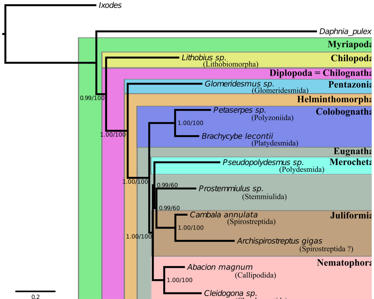
Figure 1. Phylogeny recovered from Bayesian inference conducted by the program Phylobayes. The traditional clades above the ordinal level are indicated by boxes. Support values are posterior probabilities/maximum likelihood bootstrap values from the RAxML analysis.
