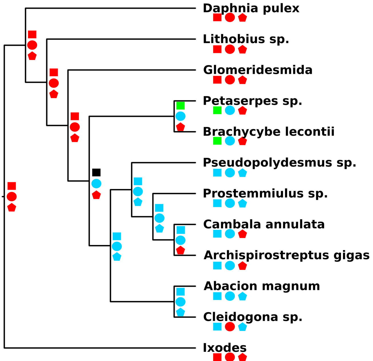
Figure 3. Ancestral character state reconstructions of features relating to millipede gonopods, ozopores, and spinnerets. The phylogeny obtained from phyllobayes imported into Mesquite and states were reconstructed under a parsimony model. Squares correspond to gonopods (red = none, green = ninth and tenth legs pairs, blue = eighth and ninth leg pairs, black = ambiguous). Circles correspond to the presence of millipede ozopores (red = none and blue = present). Pentagons correspond to millipede spinnerets (red = none and blue = present).
