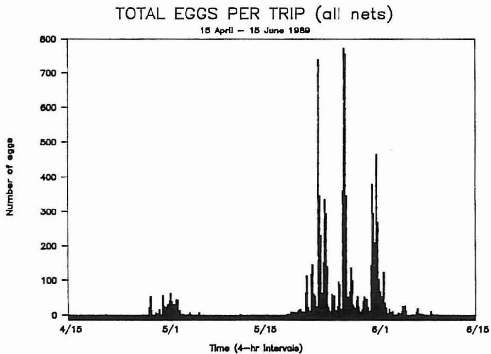
Figure 6. Number of striped bass eggs collected in all nets during each trip, and corresponding water temperatures (°C) at Barnhill's Landing, NC, for the period 15 April to 15 June 1989.
