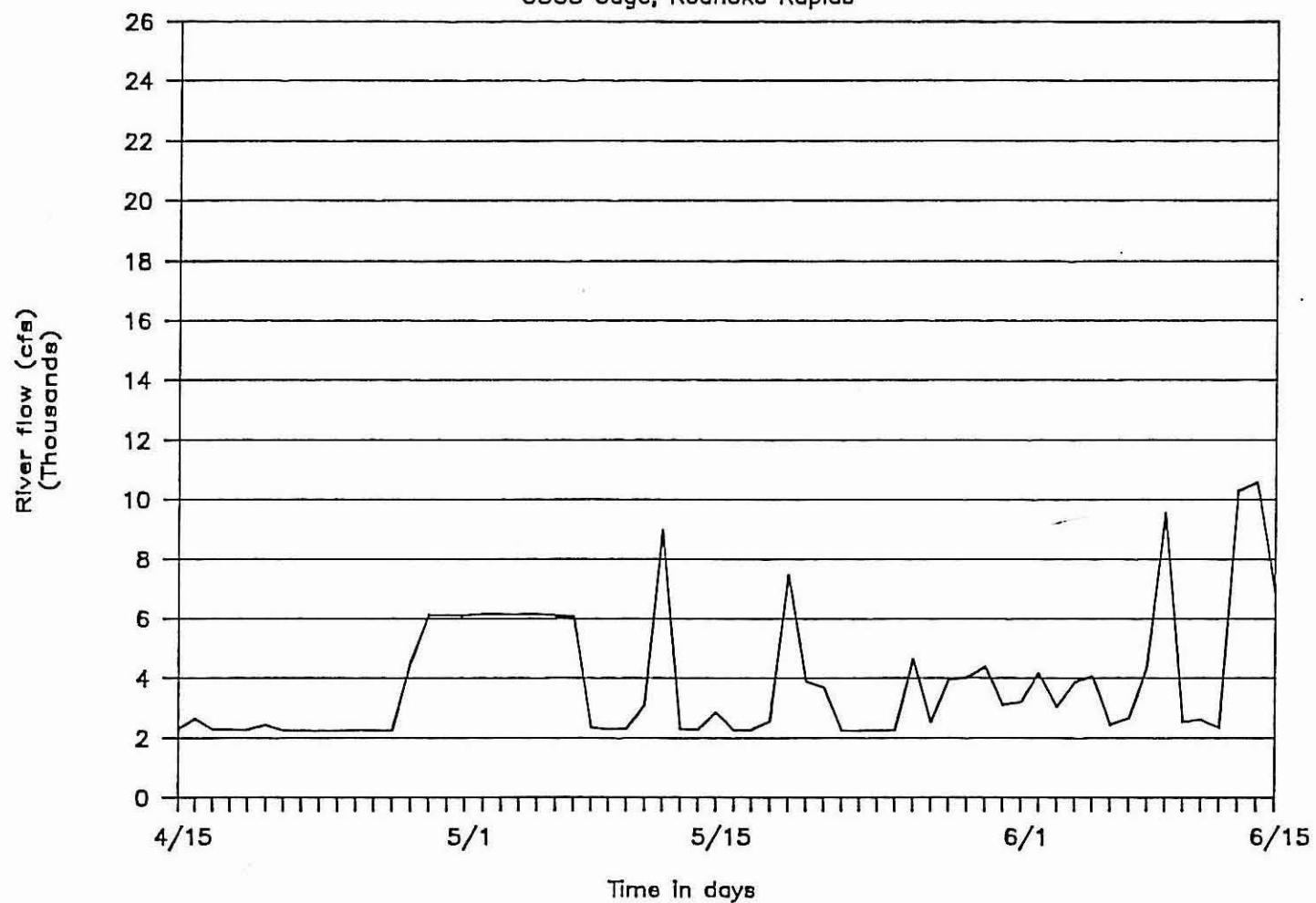
Figure 19. Average daily flow (cfs) of the Roanoke River for the period 15 April to 15 June 1981 (USGS data).
