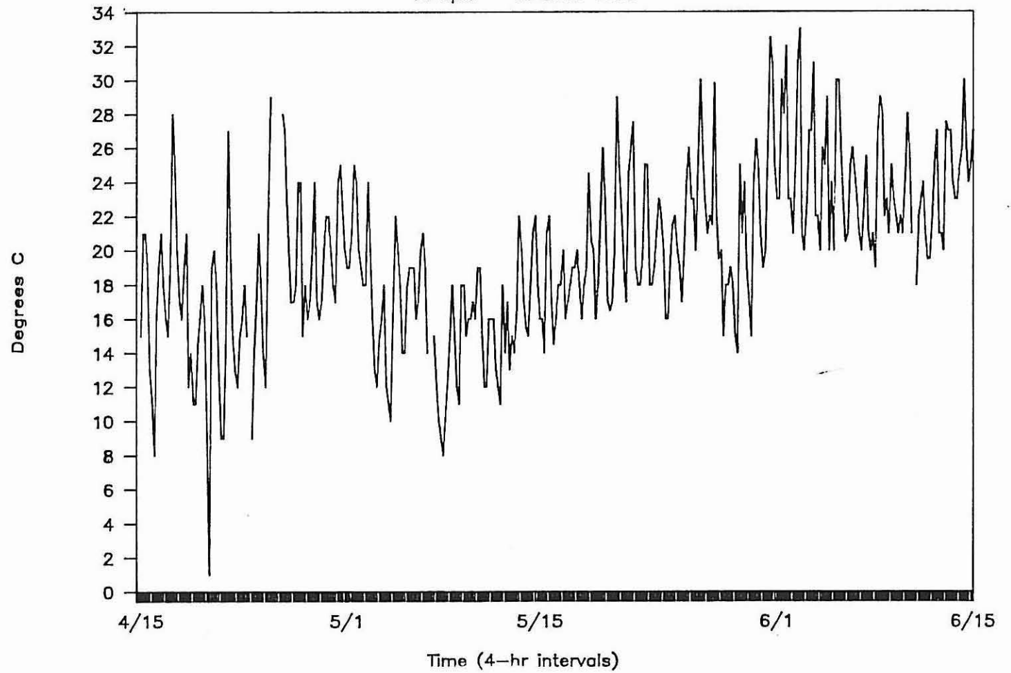
Figure 7. Air temperature (°C) measured at Barnhill's Landing, NC, for the period 15 April to 15 June 1989.
