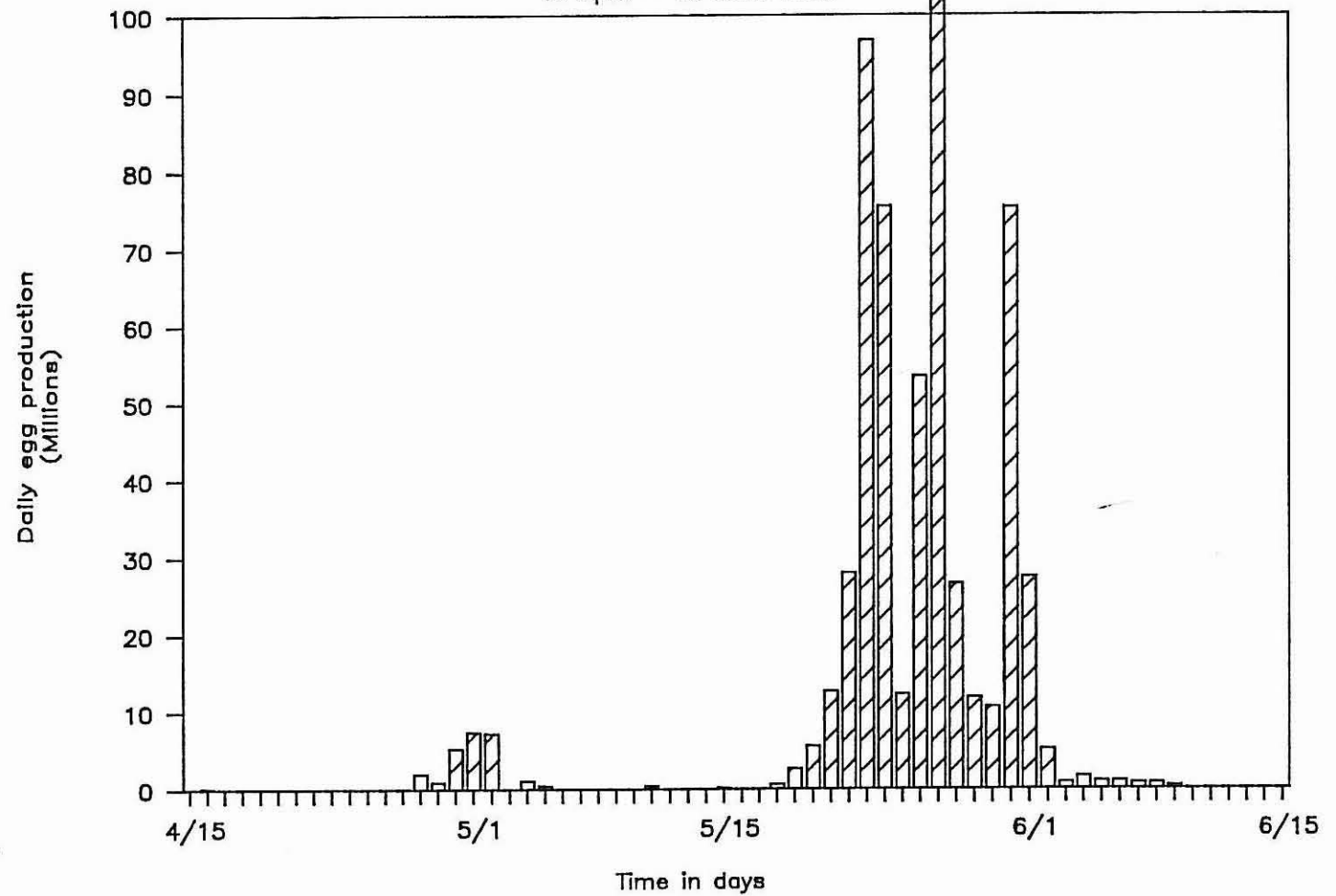
Figure 3. Estimated daily production of striped bass eggs in the Roanoke River based on samples collected at Barnhill's Landing, NC, for the period 15 April to 15 June 1989.
