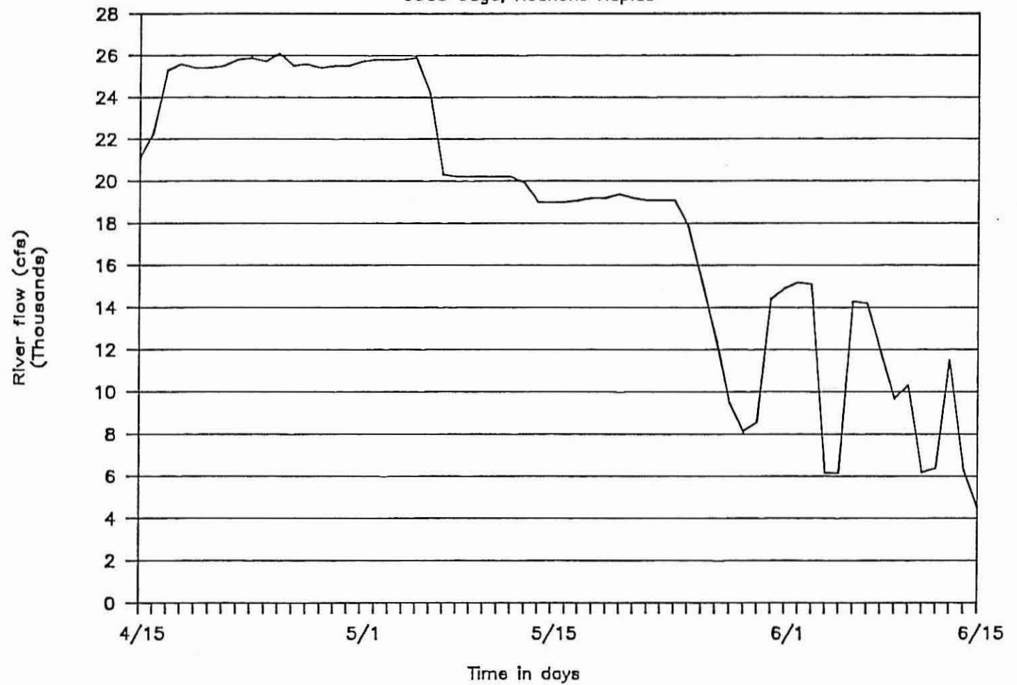
Figure 22. Average daily flow (cfs) of the Roanoke River for the period 15 April to 15 June 1983 (USGS data).
