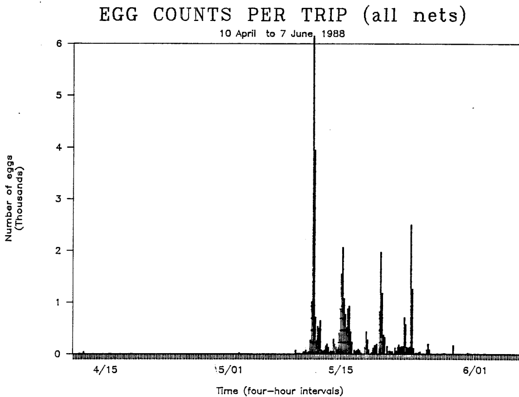
Figure 5. Number of striped bass eggs collected in all nets during each trip, and corresponding water temperatures (oC), at Pollocks Ferry, NC, in 1988.
