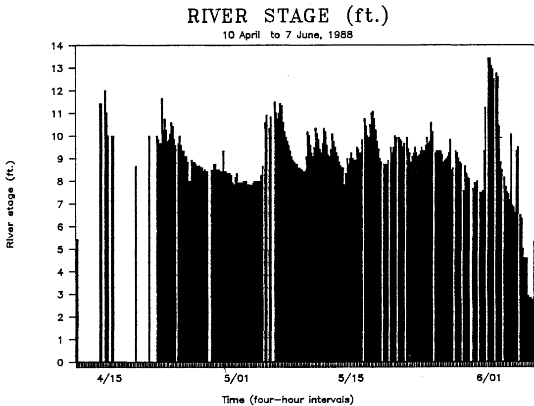
Figure 8. Hourly flow of the Roanoke River (cfs) below the Roanoke Rapids Dam (USGS gage) and relative change in river stage (ft.) at Pollocks Ferry, NC, for the period 10 April to 7 June 1988. Unfilled bars indicate no information available.
