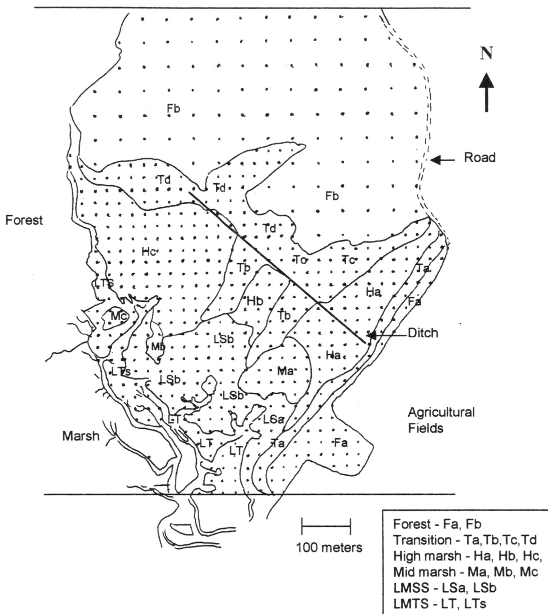
Figure 3b. Map of Phillips Creek displays spatial scale of the grid used to plot potential sampling points across zones. Legend shows stratification of zones. Legend abbreviations: LMSS = low marsh short-form Spartina alterniflora and LMTS = low marsh tall-form Spartina alterniflora
