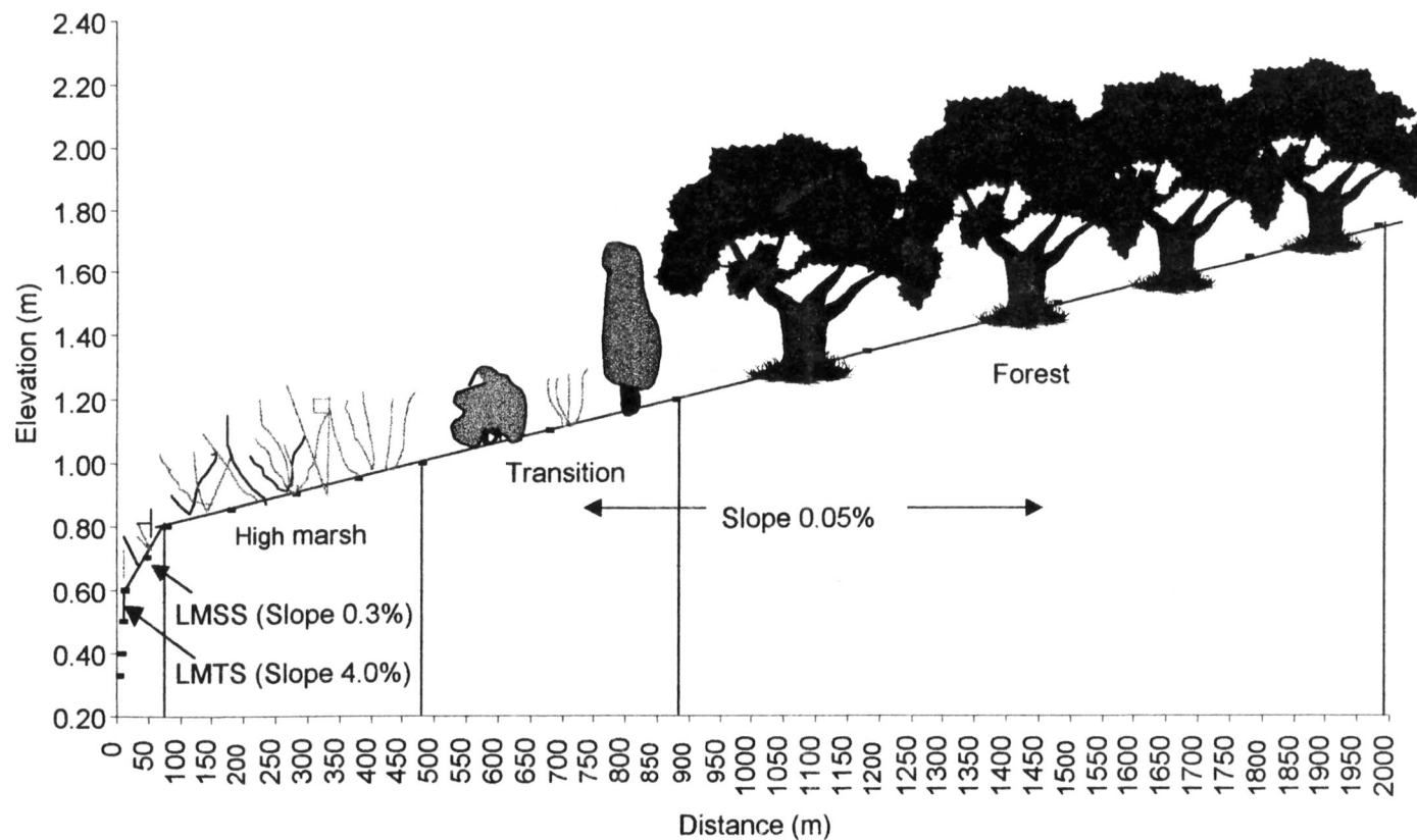
Figure 20a. Profile of Phillip Creek gentle slope at present year 2000. Zone abbreviations: LMSS = low marsh short-form Spartina alterniflora and LMTS = low marsh tall-form S. alterniflora .
