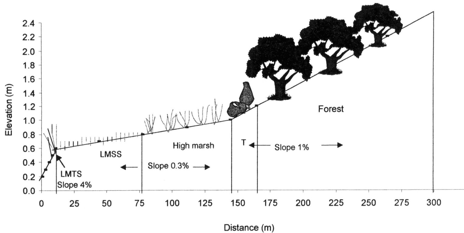
Figure 19a. Profile of Phillips Creek steep slope at present year 2000. LMTS = low marsh tall-form Spartina alterniflora , LMSS = low marsh short-form S. alterniflora , and T= transition.
