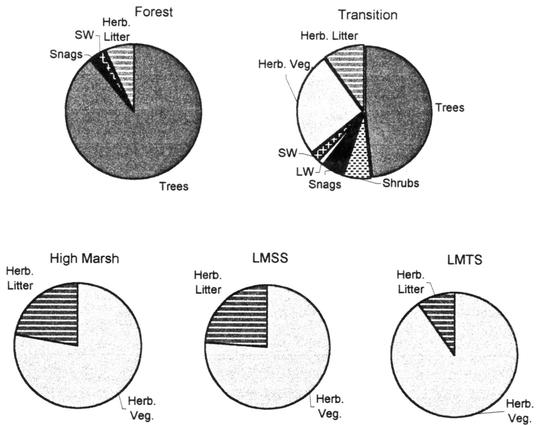
Figure 13. Distribution of vegetation mass within each zone. Any component less than 1% was not represented. LMSS = low marsh short-form S. alterniflora , and LMTS = low marsh tall-form S. alterniflora . SW = small wood detritus, LW = large wood detritus, and Herb.Veg. = herbaceous vegetation.
