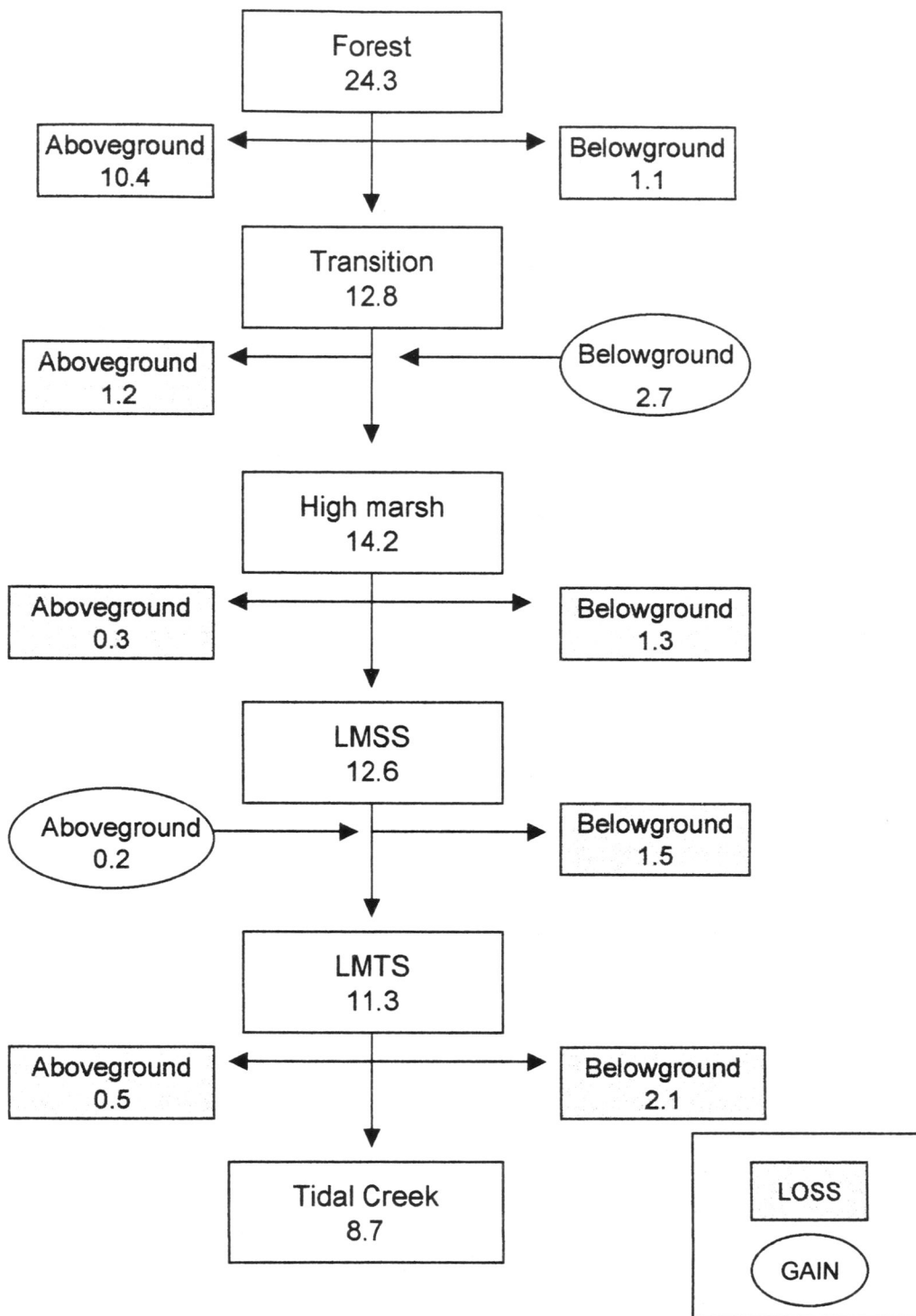
Figure 18. Organic carbon (kg/m 2 ) losses and gains with ecosystem state change along a continuum from forest to tidal creek. LMSS = low marsh short-form Spartina alterniflora and LMTS = low marsh tall-form S. alterniflora .
