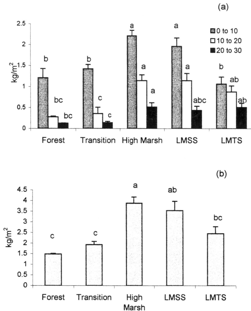
Figure 14. (a) Macroorganic matter (MOM) carbon mass for three soil depths ( F_{(4,52)} , P < 0.02 ) and (b) MOM carbon mass for total 30 cm depth ( F_{(4, 53)} , P = 0.000 ). Bar graphs are shown with standard error bars. Significant differences are indicated by different letters above the bars. LMSS = low marsh short-form Spartina alterniflora and LMTS = low marsh tall-form S. alterniflora .
