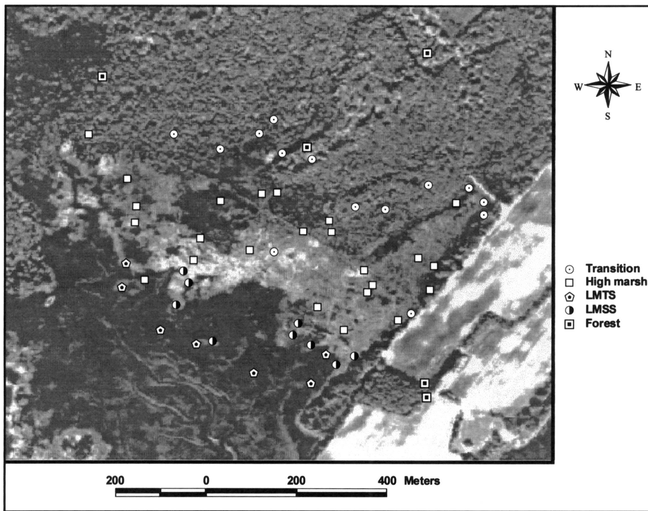
Figure 7. Georeferenced USDA (1990) aerial photograph of Phillips Creek study area displaying sample sites within all zones, except the tidal creek.
