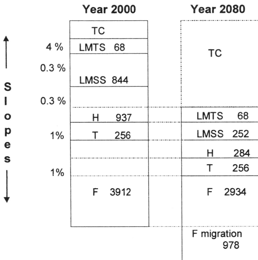
Figure 21. Projected state change following 80 y of 5 mm/y sea level rise for Phillips Creek steep profile. Original and future carbon stocks (kg/zone) are shown for marsh to forest zones along a 1 m wide transect. All zones migrate, but LMSS and H migrate up a steeper slope and loss of zone area occurs. Approximately 25% of the old forest stock has turned over. TC = tidal creek, LMTS = low marsh tall-form Spartina alterniflora , LMSS = low marsh short-form S. alterniflora , H = high marsh, T = transition, and F = forest.
