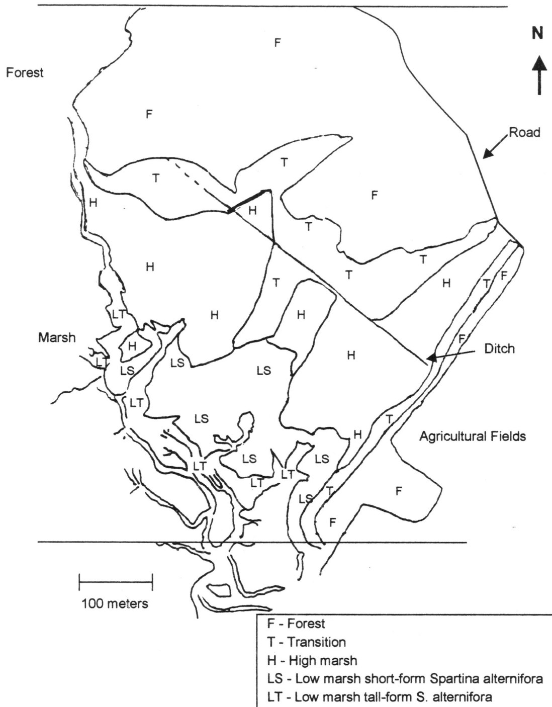
Figure 4. Revised map of Phillips Creek shown with adjusted zone boundaries.
