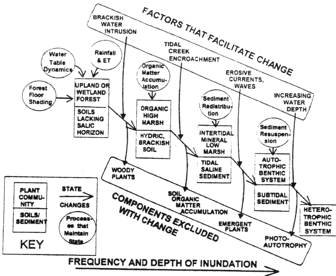
Figure 1. Conceptual model of the five states and four transitions from terrestrial forest to heterotrophic sediment. Factors that facilitate change appear at the top and components excluded with state change appear at the bottom. From Brinson et al. (1995).
