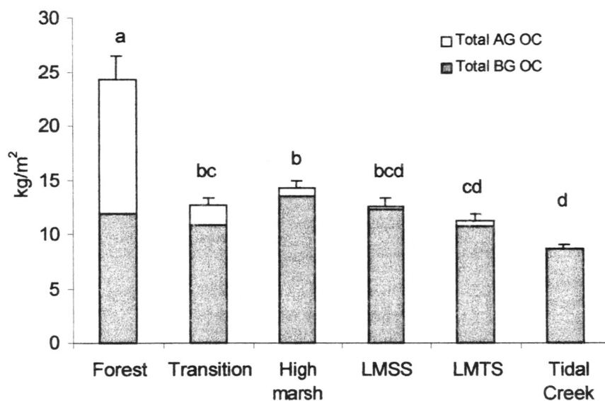
Figure 17. Sum of total above and belowground organic carbon compared across zones. Shown with standard error bars. Significance indicated by different letters above the bars ( F_{(5,57)} , P = 0.0000 ). Zone abbreviations are explained in Figure 16.
