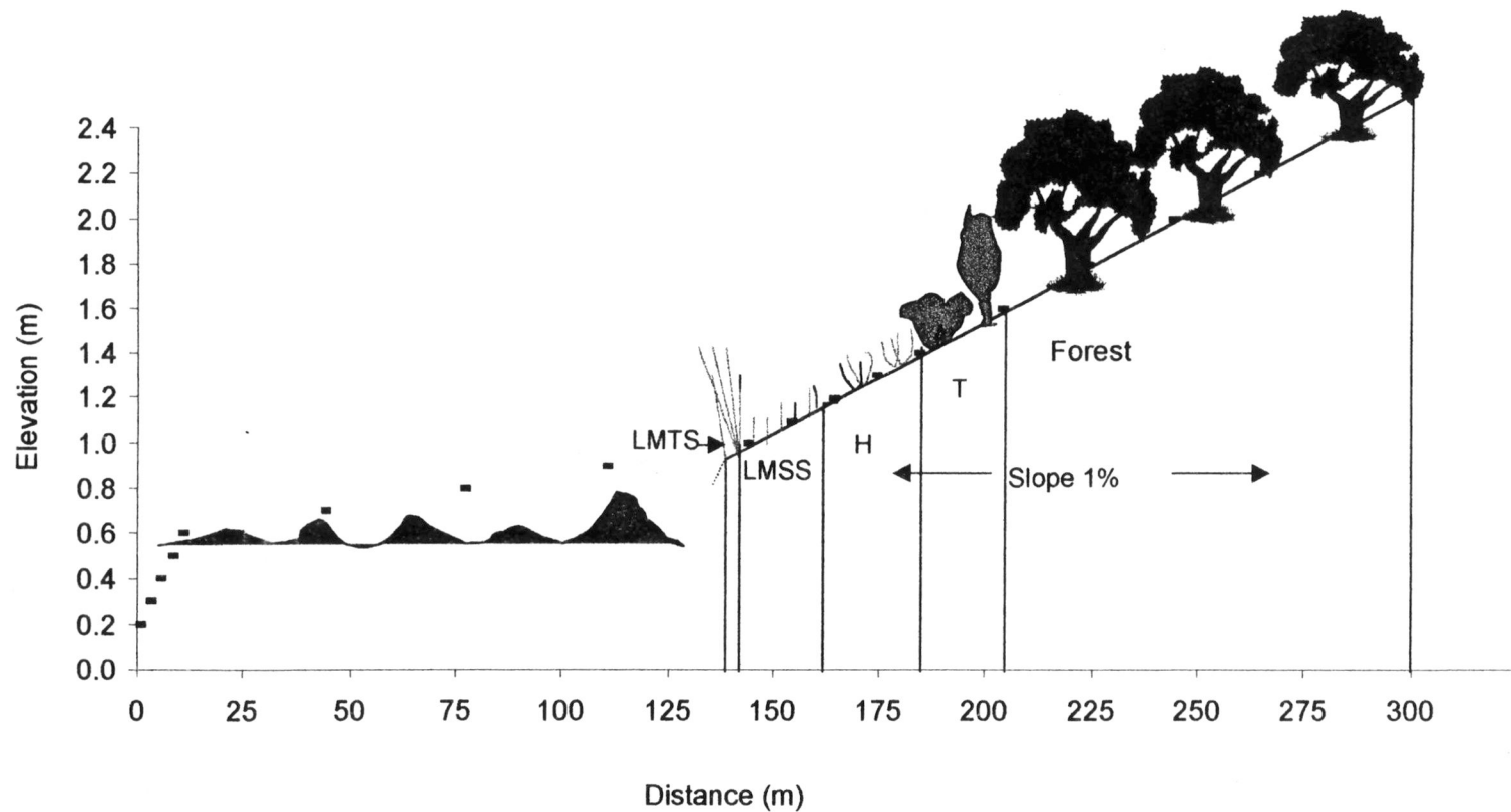
Figure 19b. Profile of Phillips Creek steep slope at year 2080 after a 5 mm/y sea level rise. Zone abbreviations: H = high marsh, LMSS = low marsh short-form Spartina alterniflora , and LMTS = low marsh tall-form S. alterniflora .
