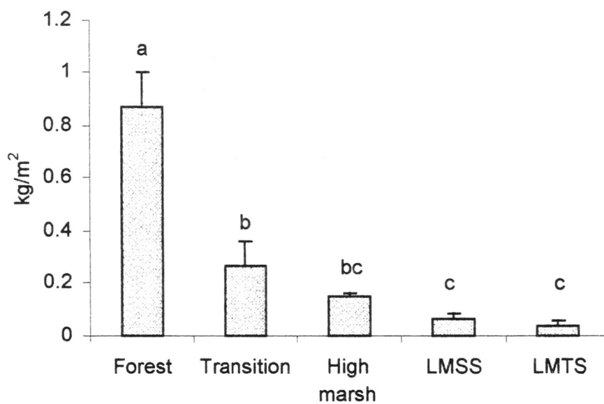
Figure 10. Organic carbon mass of herbaceous litter across zones. Bars with the same letter are not significantly different ( F_{(4,55)} , p = 0.0000 ).
