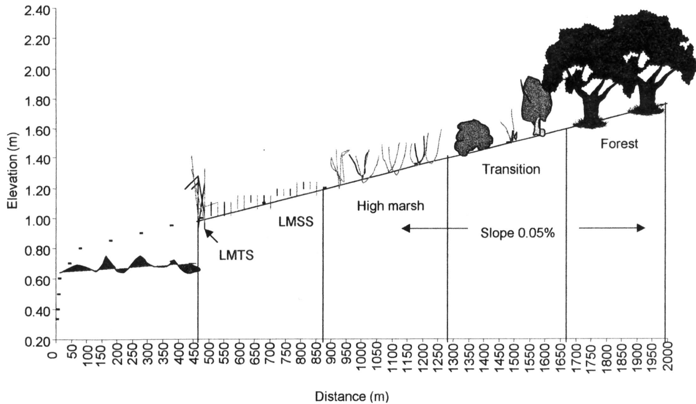
Figure 20b. Profile of Phillips Creek gentle slope at year 2080 after a 5 mm/y sea level rise. Zone abbreviations: LMSS = low marsh short-form Spartina alterniflora and LMTS = low marsh tall-form S. alterniflora .
