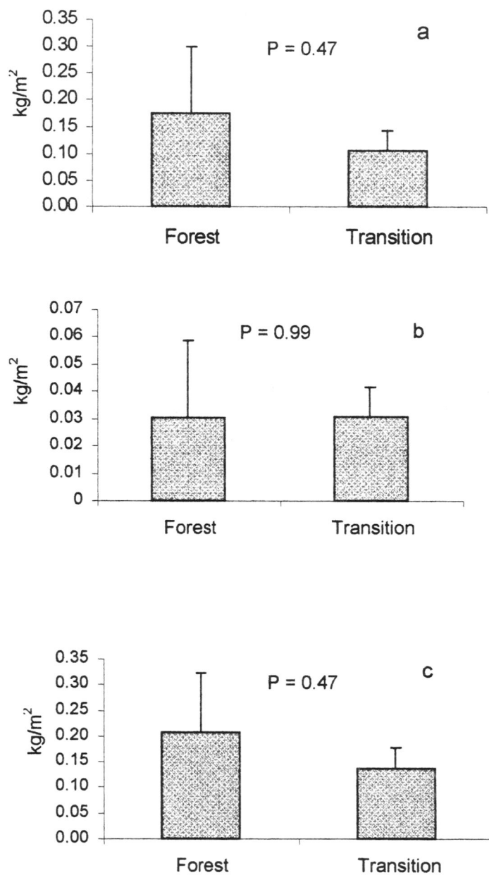
Figure 11. Average organic carbon mass of (a) snags, (b) large wood detritus, and (c) combined snags and large wood detritus of forest and transition zones. Shown with standard error bars. No significant differences with t-tests, df = 17 in all 3 categories.
