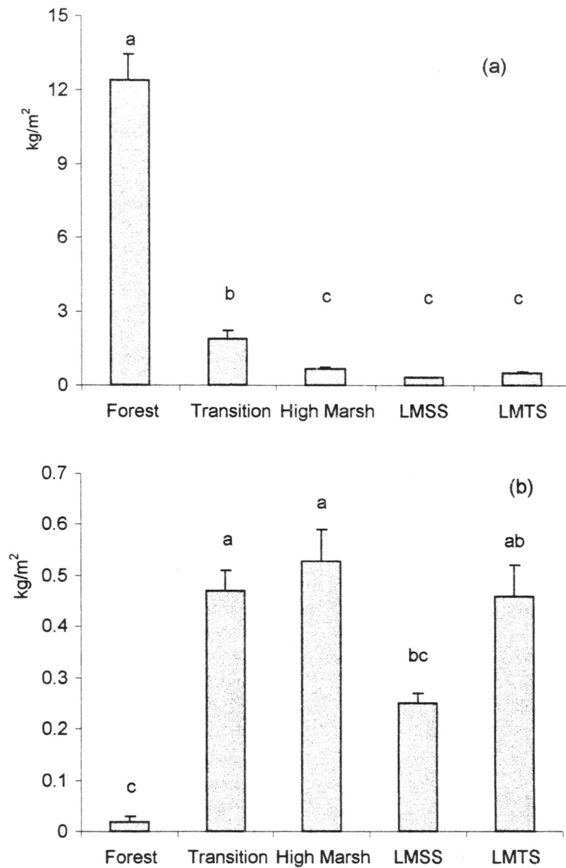
Figure 8. Organic carbon mass of (a) total aboveground vegetation and (b) herbaceous vegetation across zones. Shown with standard error bars. Different letters above the bars indicate significant differences ( F_{(4,55)} , P = 0.000 ). LMSS = low marsh short-form Spartina alterniflora and LMTS = low marsh tall-form S. alterniflora .
