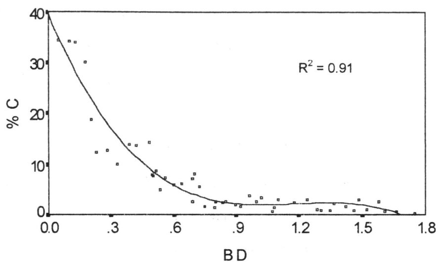
Figure 6. Cubic regression of bulk density predicting percent organic carbon.
