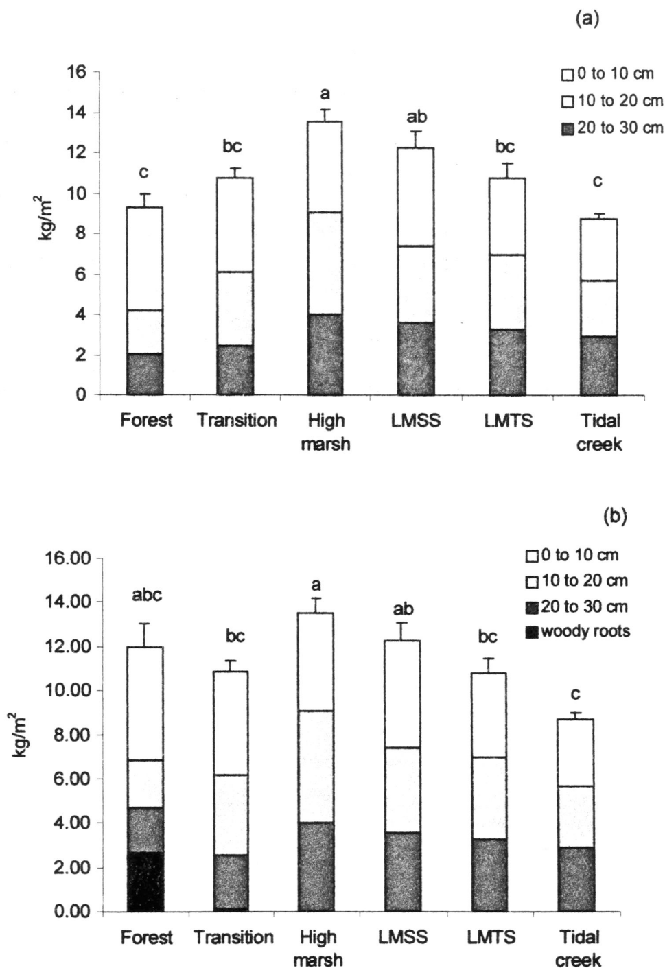
Figure 15. Belowground organic carbon from (a) 30 cm soil depth compared across zones ( F_{(5,56)} , P = 0.001 ), and (b) a grand total which is the sum of 30 cm depth and woody roots (derived from P. taeda root regression and 30-50 cm MOM cores), ( F_{(5,56)} , P = 0.009 ). Significance indicated by different letters above bars.
