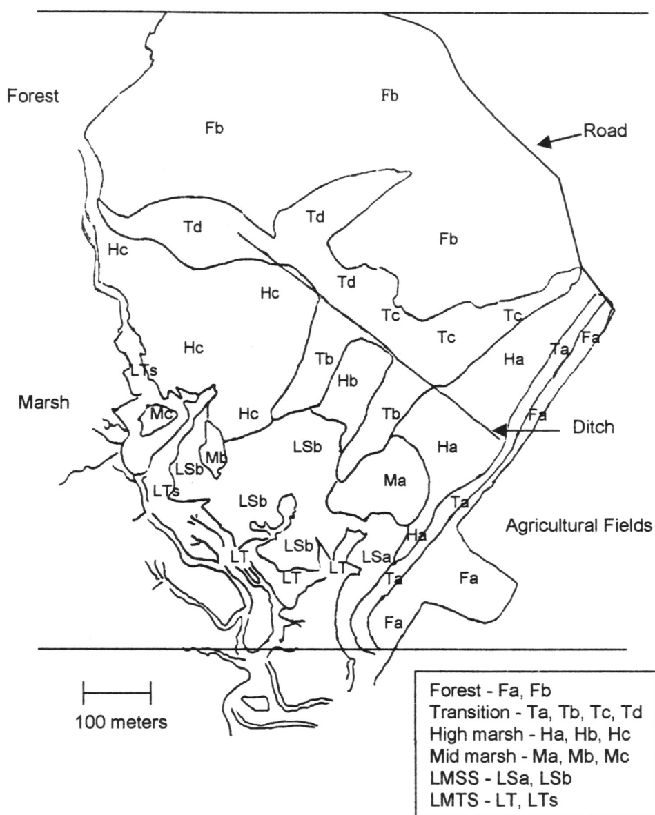
Figure 3a. Map of Phillips Creek shown with zone boundaries and stratification scheme. Capital letters denote zones and small case letters denote strata. LMSS = low marsh short-form Spartina alterniflora and LMTS = low marsh tall-form Spartina alterniflora .
