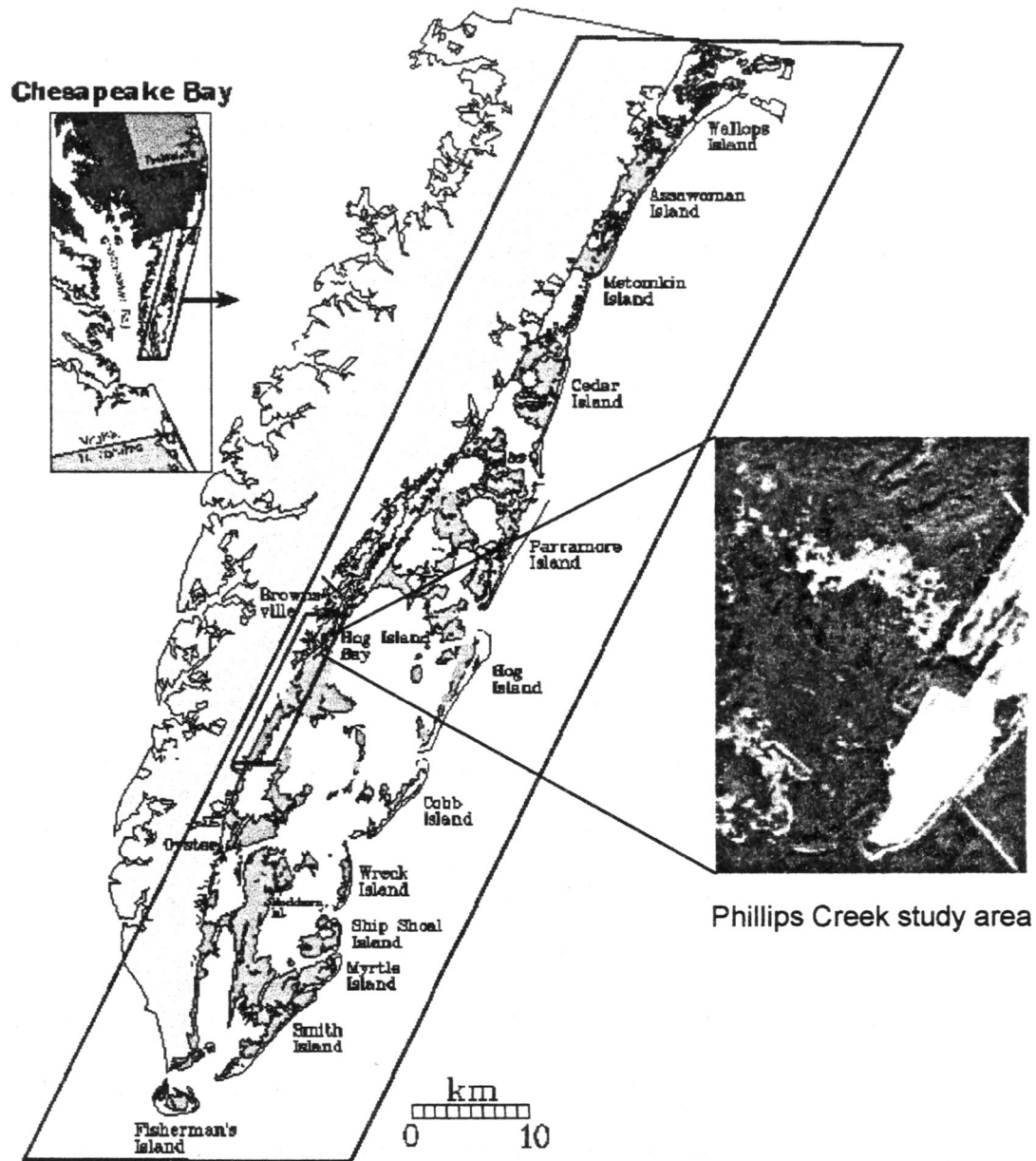
Figure 2. Phillips Creek study area is located within the Virginia Coast Reserve Long-Term Ecological Research complex. This complex is situated on the eastern shore of Virginia on the Delmarva Peninsula. Mainland marshes (small rectangle) are attached to the major land mass in contrast to lagoonal and back barrier marshes to the east.
