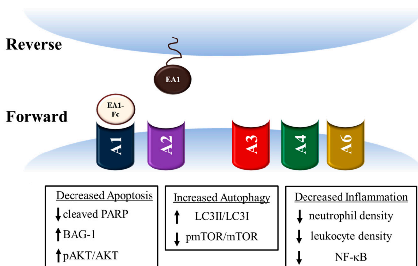
Figure 2. Potential Mechanisms of EA1-Fc Mediated Cardioprotection. Treatment with Ephrin A1-Fc (EA1-Fc) in a mouse model of myocardial infarction (MI) was shown to alter expression of five Ephrin receptors (EphA1-A4 and EphA6) as well as endogenous EA1 ligand when compared to the vehicle treated MI group. Canonical ephrin signaling regulates a wide-variety of physiological processes. The cardioprotective role of EA1-Fc may be attributed to ephrin signaling. In support of this, in the EA1-Fc MI group, indicators of decreased apoptosis, increased autophagy, and decreased inflammation were observed. The possibility also exists that EA1-Fc injection is cardioprotective through a mechanism that is not normally attributed to ephrin signaling.
